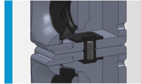
Connection of two L-Series elements by an M10 thread bolt and washer. The two elements can be faced in different horizontal directions (08149/bolt).
