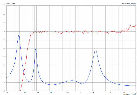
Frequency Response with Preset + Impedance
